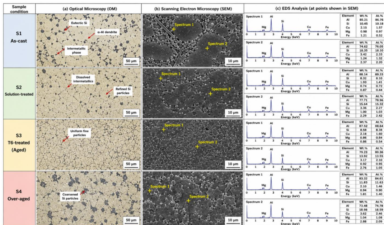
Fig. 2. Microstructural characterization of aluminum piston alloys under different heat-treatment conditions: (a) optical microscopy (OM) images showing the evolution of \alpha -Al dendrites, eutectic silicon particles, and intermetallic phases; (b) SEM micrographs illustrating the morphological changes and distribution of secondary phases; and (c) EDS spectra and elemental compositions of representative regions for S1 (as-cast), S2 (solution-treated), S3 (T6-treated), and S4 (over-aged) samples.
