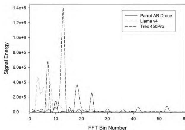
Figure 7: Small Rotorcraft Identifiers
