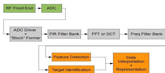
Figure 5. An overview of the data pipeline.
