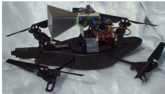
Figure 4. Radar-equipped swarm drone.
